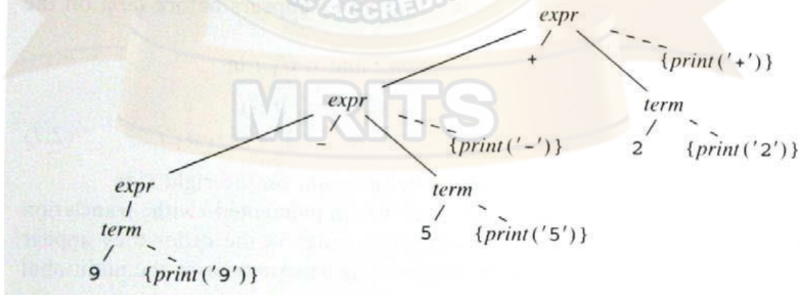
Fig 2.9. Actions translating 9-5+2 into 95-2+.
